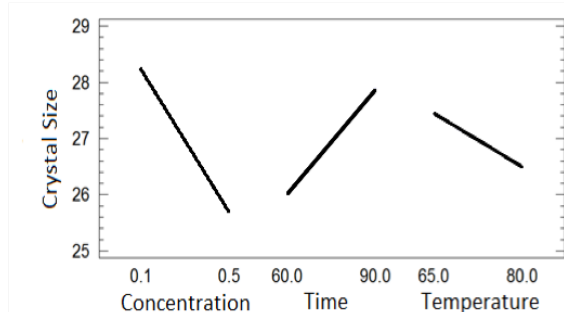
Fig. 5. Effect of concentration, time and temperature on crystal size.
