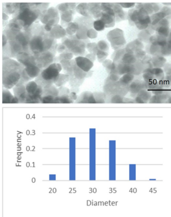
Fig. 3. TEM micrograph and their histogram of sample obtained at 65 °C, 60 minutes of reaction time and 0.5 M of zinc nitrate.
