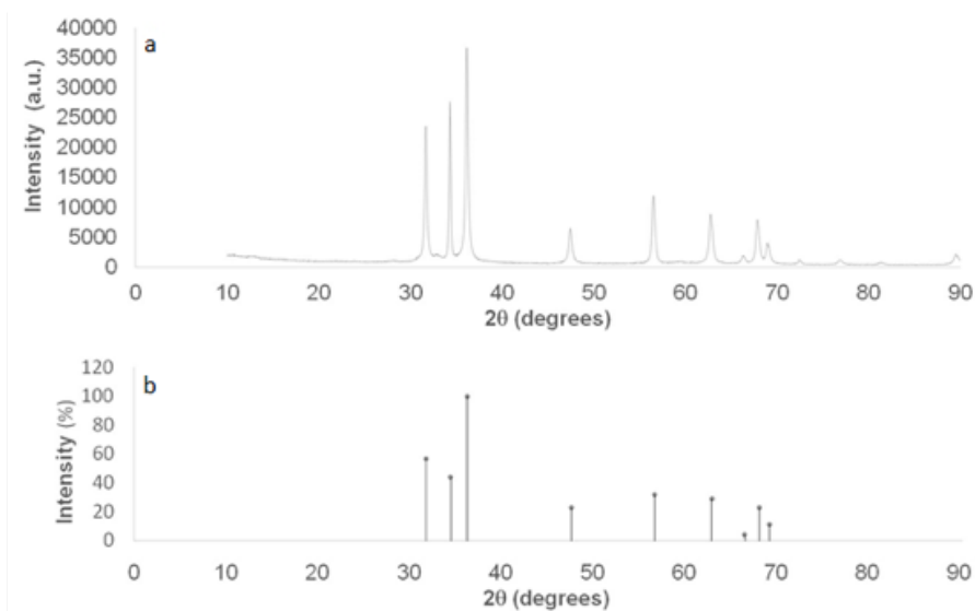
Fig. 2. XRD pattern of ZnO. a) Powder synthesized at 80 °C. b) ICDD No. 36-1451.
