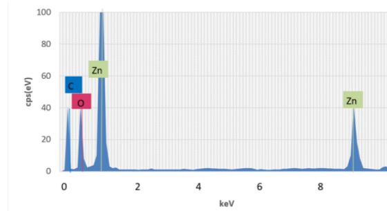
Fig. 1. EDS spectra of zinc oxide nanoparticles.
