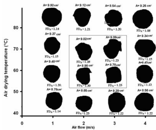
Fig. 5. Binary images of projected area of samples dried under different conditions. Images within square are those for which FD_A was higher.
