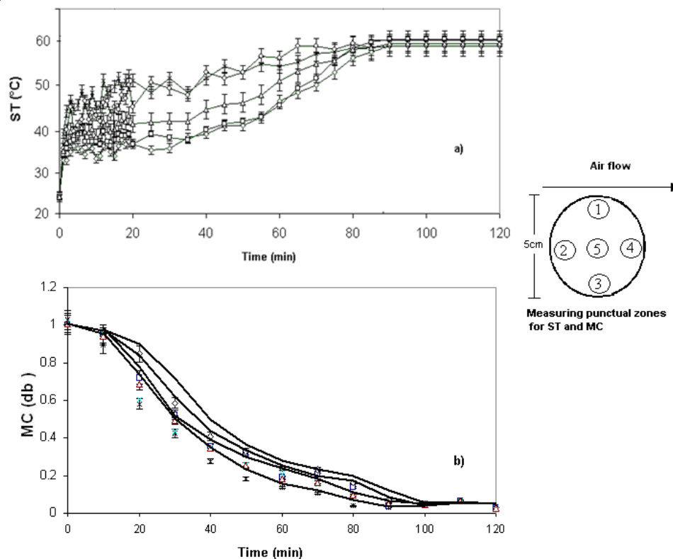
Fig. 6. Distribution of ST and moisture content for punctual zones during drying at 60°C and 2m/s. O ZONE 1, * ZONE 2, △ ZONE 3, ◇ ZONE 4 and □ ZONE 5.
