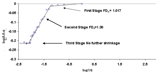
Fig. 3. \text{Log}(A/A_0) v_s \text{log}(1/t) ; drying conditions: 60°C and 2m/s.
