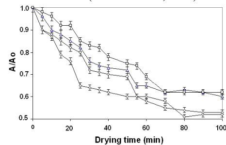
Fig. 2. A/Ao kinetics at different drying conditions ( \square 80°C 2m/s, \diamond 70°C 2m/s, \circ 60°C 2m/s, \Delta 50°C 2m/s).
