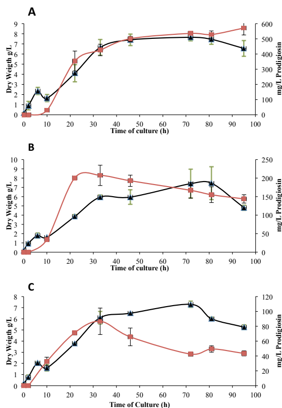
Fig. 7. Growth and prodigiosin production kinetics for S. marcescens using of three different starches as carbon sources. A. Polartex® instant starch; B. Stabitex® instant starch; C. Soluble starch. (■) Prodigiosin production curve (right axis); (▲) Bacterial growth curve (left axis).
