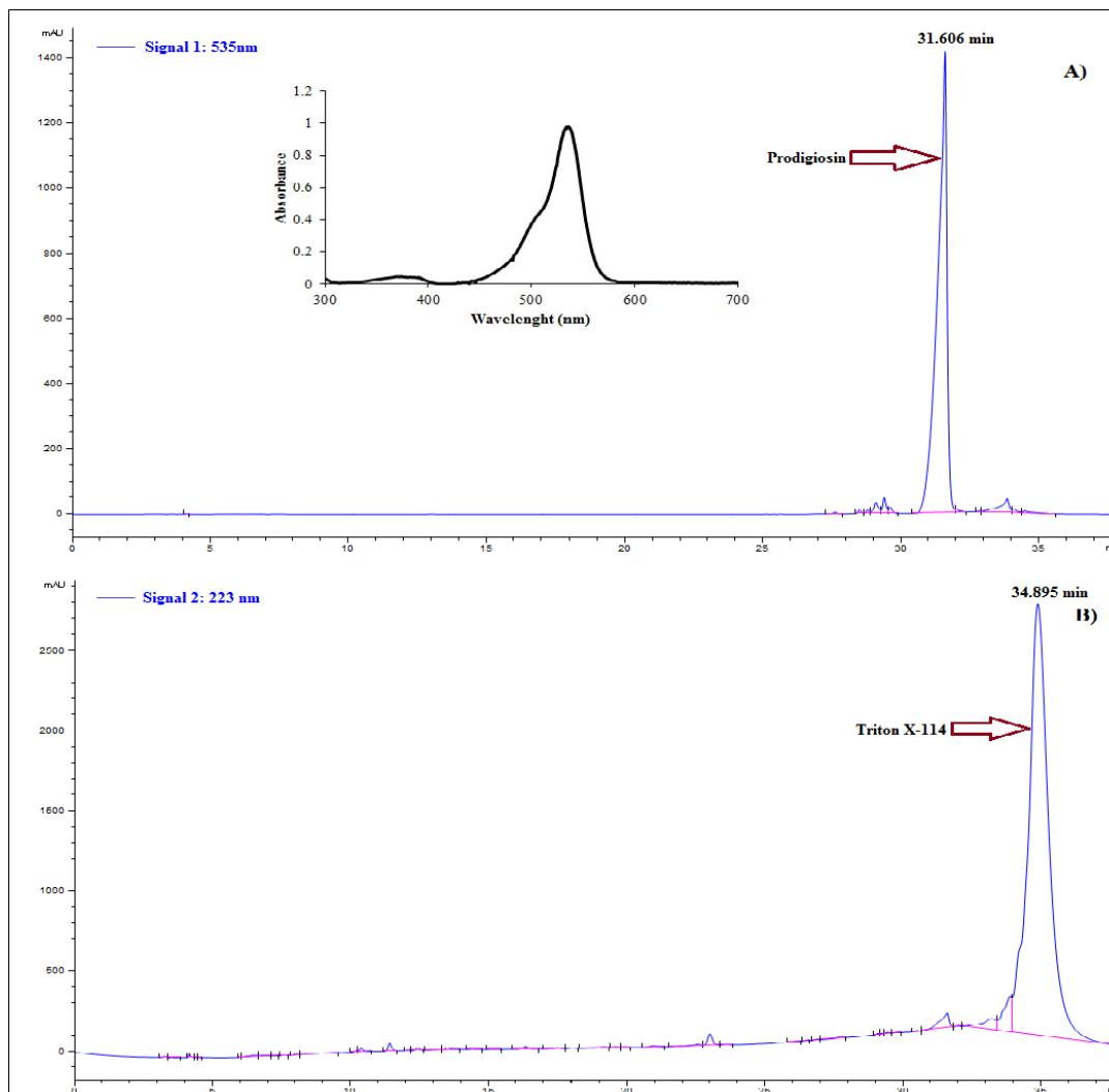
Fig. 1. Chromatogram obtained from reverse micelle extraction method. A) The single peak obtained at 535 nm represents the extracted prodigiosin ( t_r = 31.6 min), absorbance spectrum of the peak at 31.6 min is presented in the left, B) the mayor peak obtained by detection at 223 nm correspond to Triton X-114 the main contaminant ( t_r = 34.89 ).
