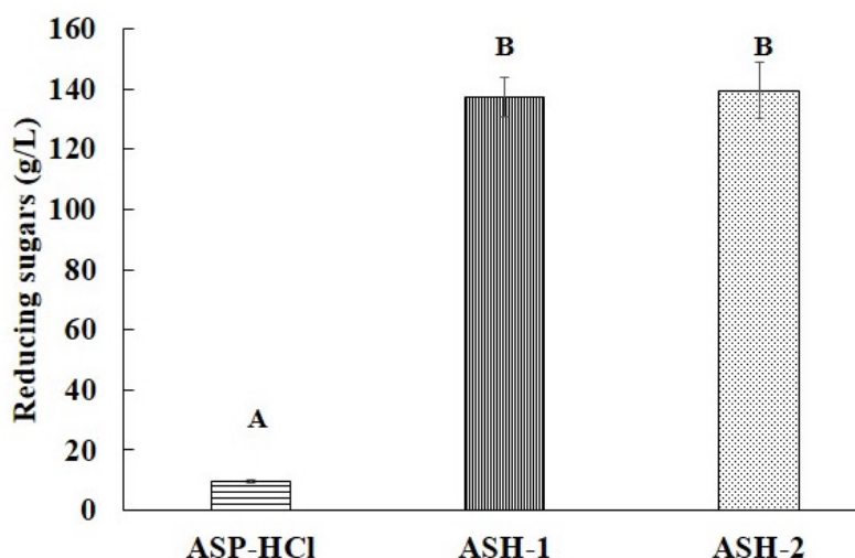
Fig. 3. Reducing sugars concentration during acid-autoclave hydrolysis of avocado seed powder. Avocado seed powder with HCl (ASP-HCl), avocado seed hydrolysed treatment one (ASH-1), avocado seed hydrolysed treatment two (ASH-2). Means with different letters are significantly different. Tukey-Kramer Test, \alpha \leq 0.05 , (NCSS, 2007).
